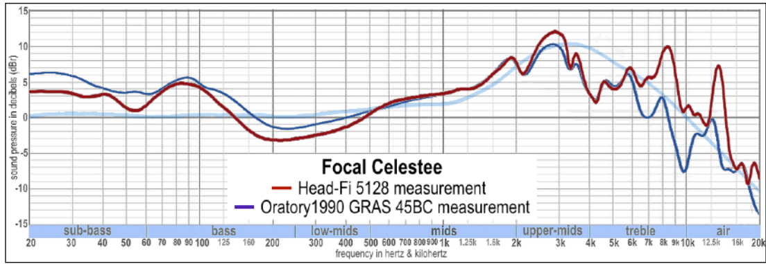
Fig. A9: Focal Celestee (closed-back dynamic driver)
