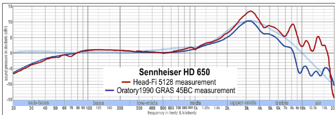
Fig. A5: Sennheiser HD 650 (open-back dynamic driver)
