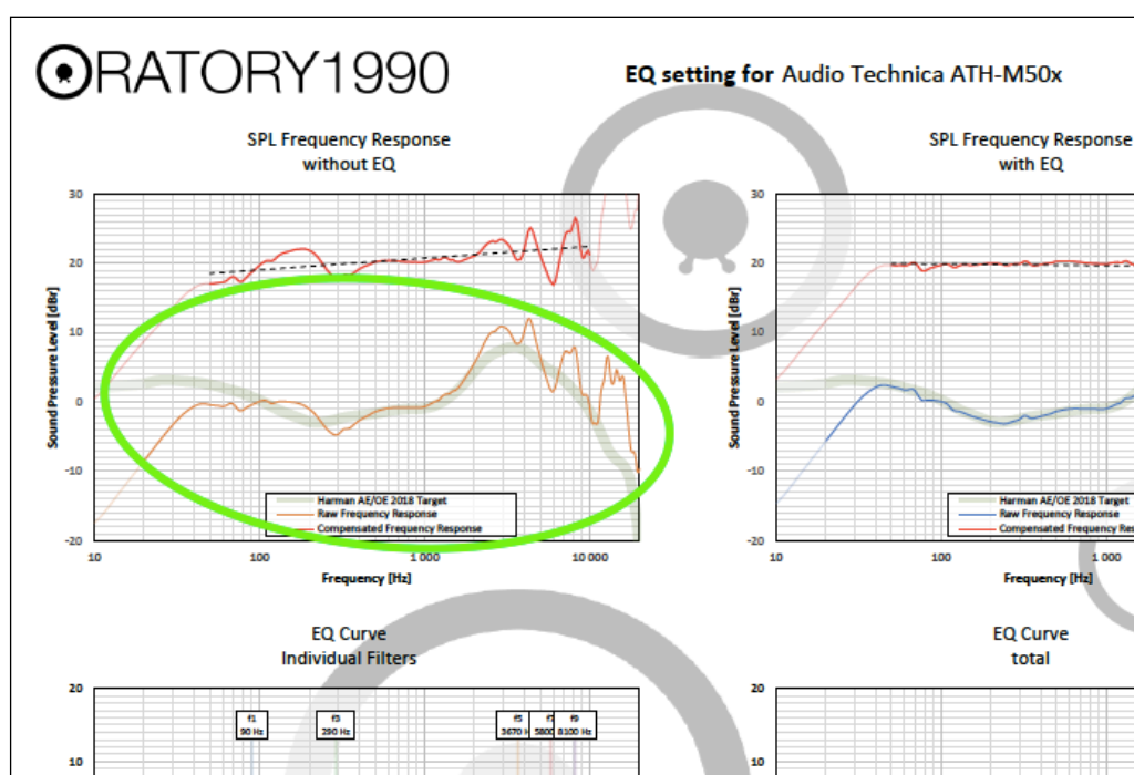
Fig. 11: Oratory1990 EQ database page for M50x with FR graph circled in green
