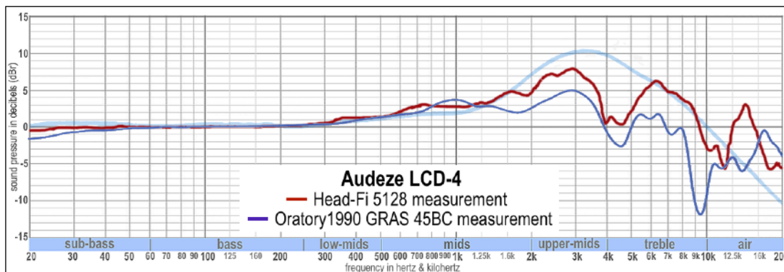
Fig. A8: Audeze LCD-4 (open-back planar magnetic driver)
