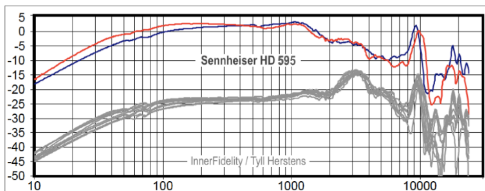
Fig. 26: InnerFidelity graph of the Sennheiser HD 595 showing multiple re-seats plus left and right ear responses
