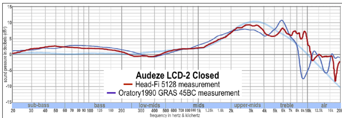
Fig. A7: Audeze LCD-2 Closed (closed-back planar magnetic driver)
