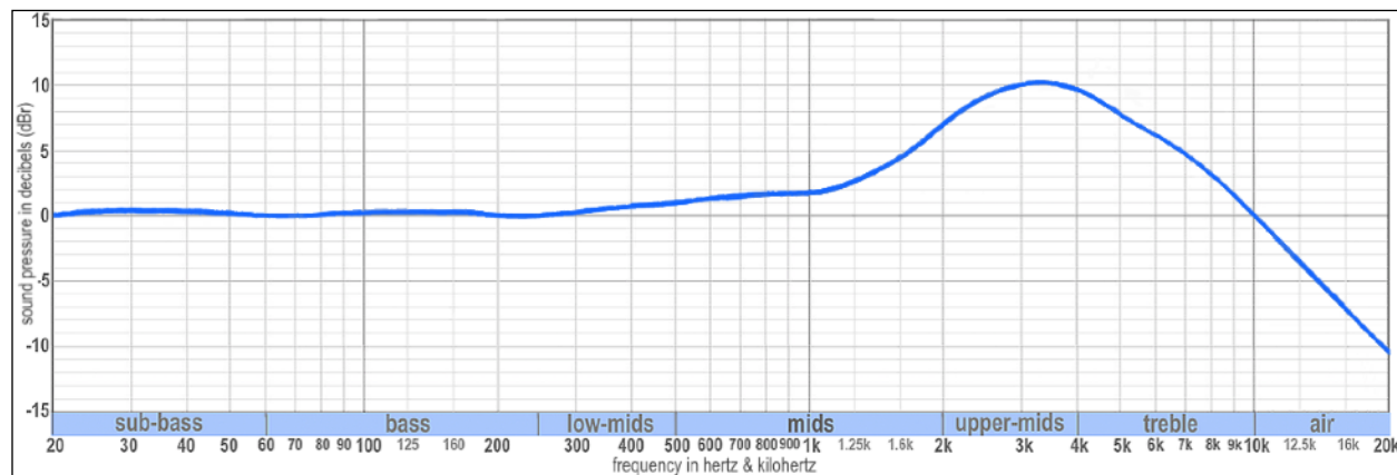
Fig. 6: Oratory Optimum HiFi over-ear headphone neutrality curve
