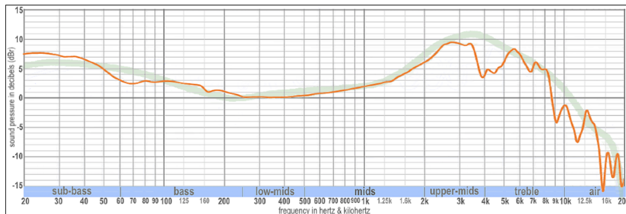
Fig. 13: Oratory1990 FR graph for AKG K371
