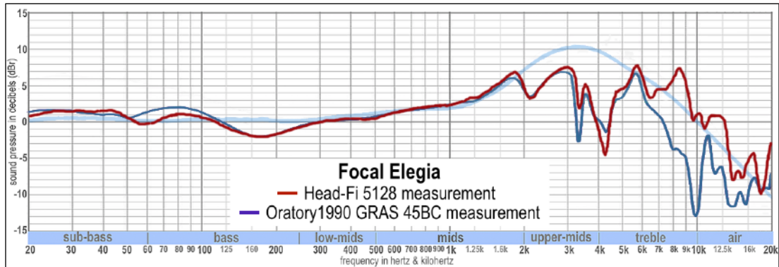
Fig. A10: Focal Elegia (closed-back dynamic driver)
