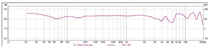
Fig. 14: MiniDSP EARS frequency response graph for AKG-K371
