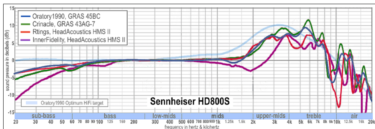
Fig. 21: four-way comparison of raw measurements of the Sennheiser HD 800S headphone
