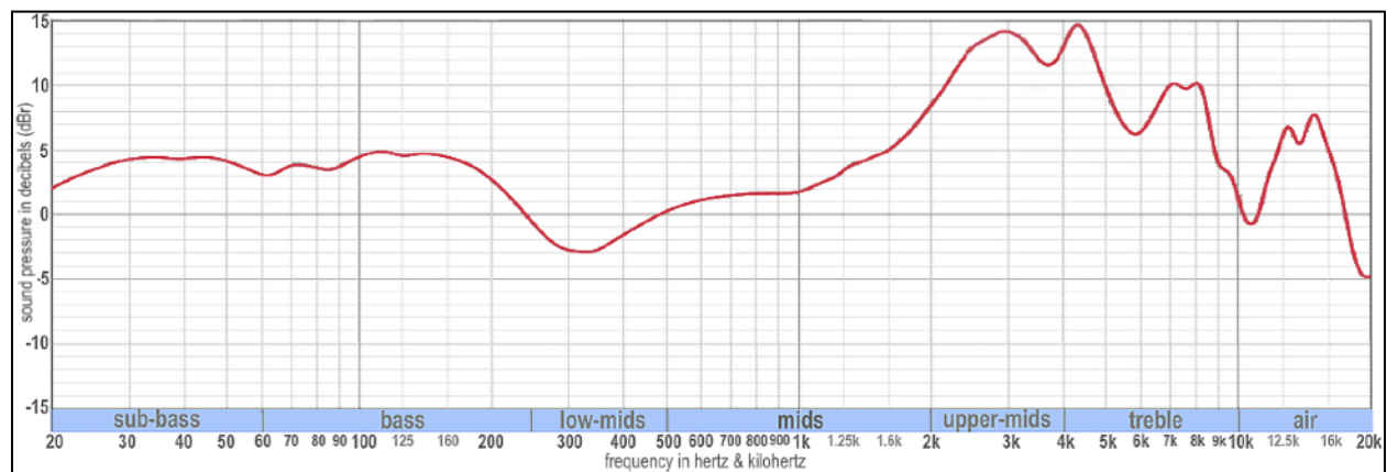
Fig. 5: Oratory1990 FR graph for the Audio-Technica ATH-M50x
