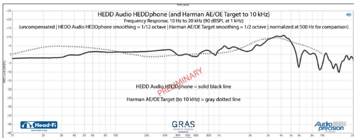
Fig. 18a: Head-fi measurements for the HEDDphone
