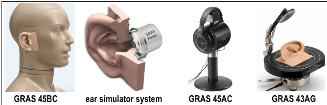
Fig. A1: current GRAS measurement systems
