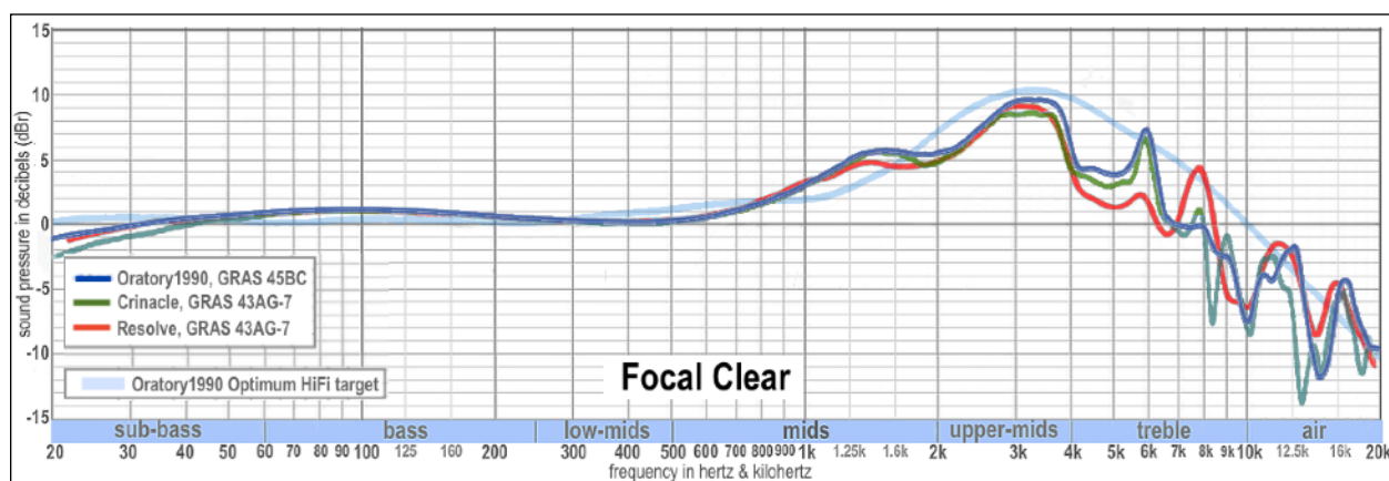
Fig. 19: three-way comparison of GRAS measurements of the Focal Clear headphone
