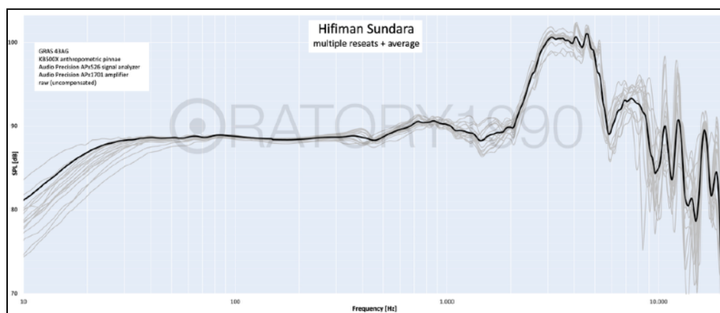
Fig. 25: Oratory1990 graph of the frequency response of a Hifiman Sundara showing multiple re-seats
