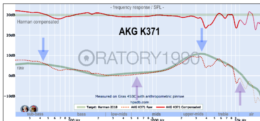
Fig. 15: AKG K371 graph morphed to straighten the Harman target curve
