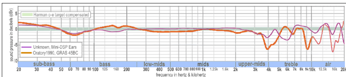
Fig. 16: compensated graph comparison: MiniDSP EARS versus GRAS 43AG for AKG-K371
