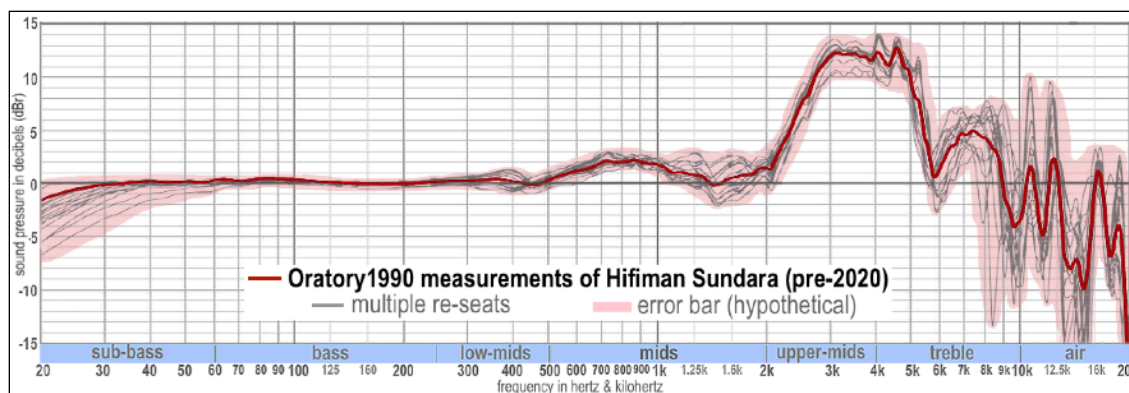
Fig. 27: Hifiman Sundara graph from Fig. 25 showing re-seating trials and (fictitious) error band
