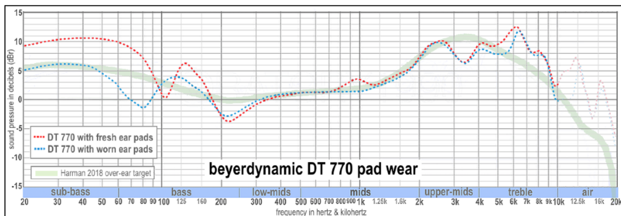
Fig. 24: effect of pad wear on the beyerdynamic DT 770 (Oratory1990 data)
