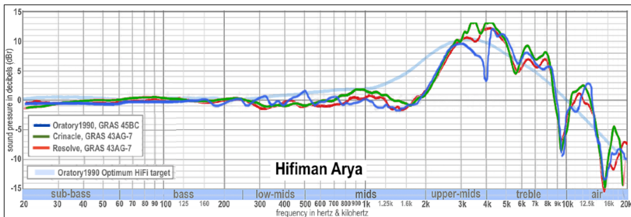
Fig. 20: three-way comparison of GRAS measurements of the Hifiman Arya headphone
