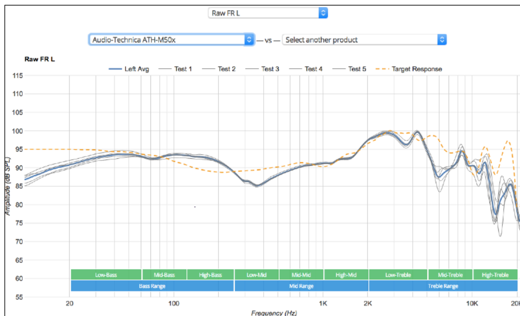
Fig. 9: rtings.com measurements for M50x
