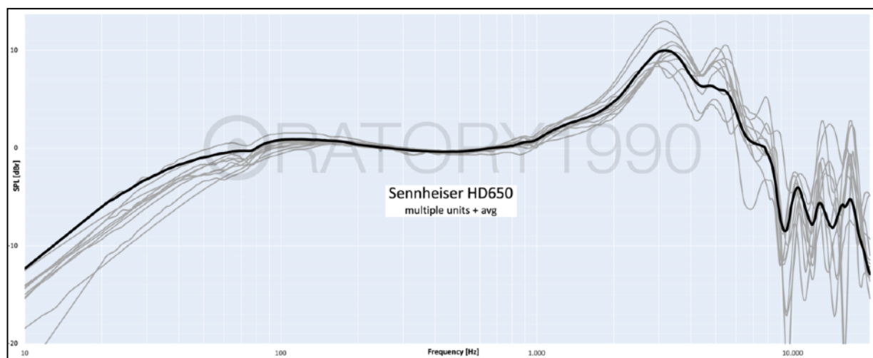
Fig. 23: different units of same headphone model (Sennheiser HD 650)
