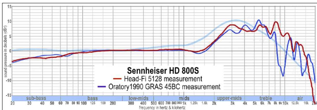
Fig. A6: Sennheiser HD 800S (open-back dynamic driver)
