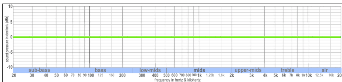
Fig. 7: subjective experience of a perfectly even loudness across the frequency range
