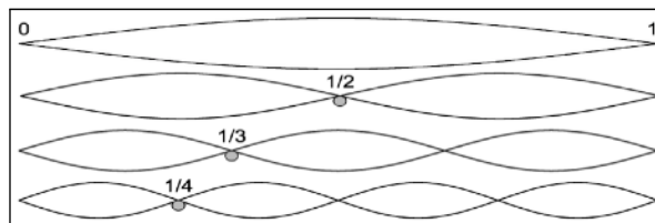
Fig. 28: first four vibrational modes
