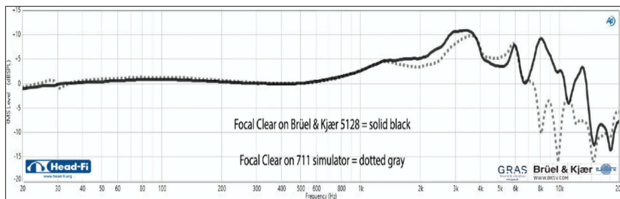
Fig. A4: Focal Clear (open-back dynamic driver) measured on 5128 (solid) and GRAS 45 (dotted)
